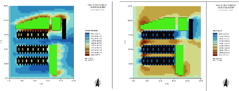
Figure 7: Envi Met Results of Relative Humidity and Wind Velocity on 22 nd May 2024.
