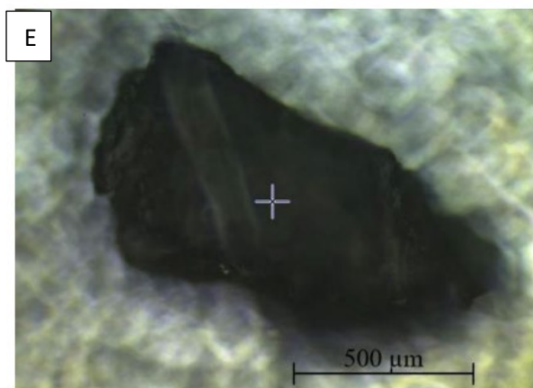
Fig 1: Shapes of Microplastic: A- Spherical, B- Fiber, C- Fragmented, D- Thin Sheet, and E- Irregular shape (Environmental and climate change Canada, 2015; Hongprasith et al., 2020)
