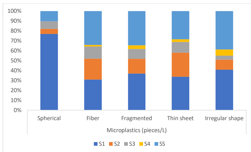
Fig 2 Classification of Microplastics (Pieces/L) in samples
