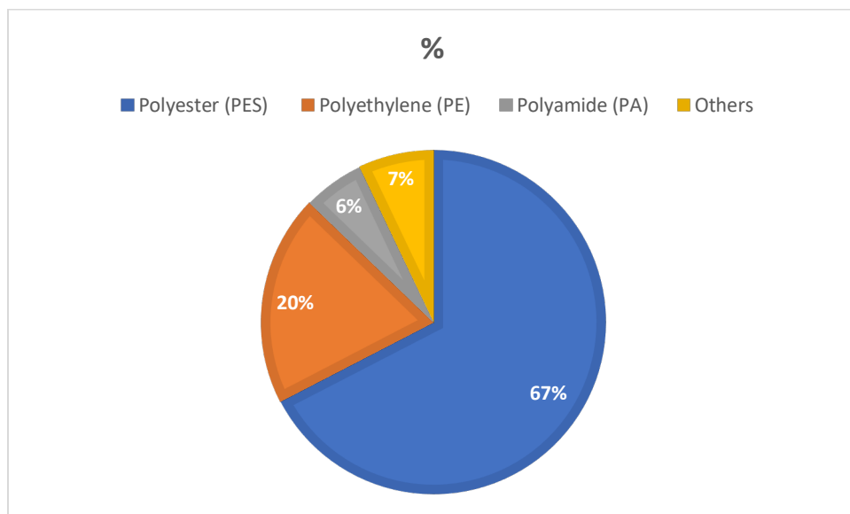
Fig 4: Type of polymer present in wastewater samples
