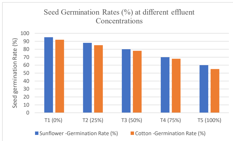
Fig. 5: Seed Germination Rates (%) at different effluent Concentrations.
