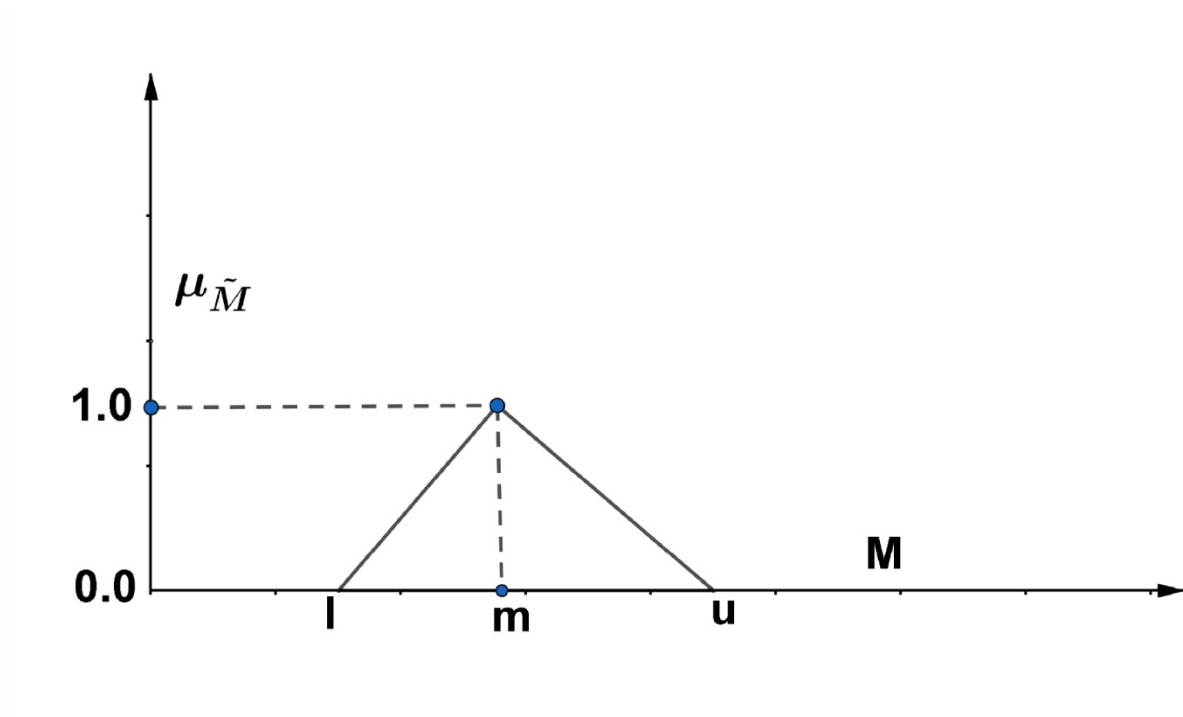
Fig. 2 Graphical representation of a triangular fuzzy membership function
