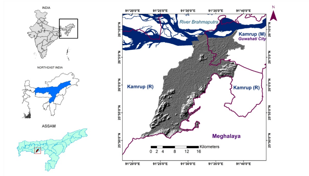
Fig. 1 SRTM DEM derived hill shade map of the area showing Rani and Chayani Barduar administrative blocks located at the southwestern fringe of the Guwahati city, Assam, India
