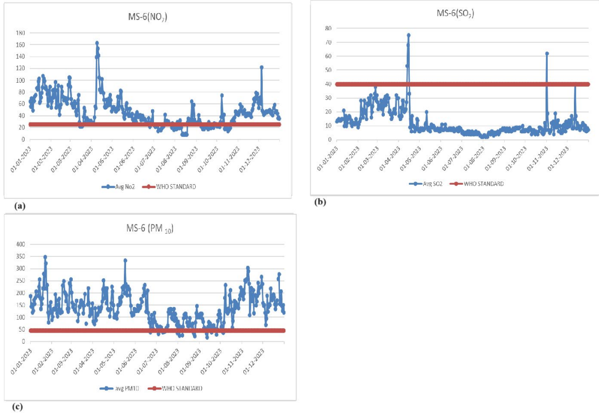
Figure 9. Comparative prediction of ground truth (a)NO 2 , (b) SO 2 and (c) PM 10 with WHO standards of MS 6
