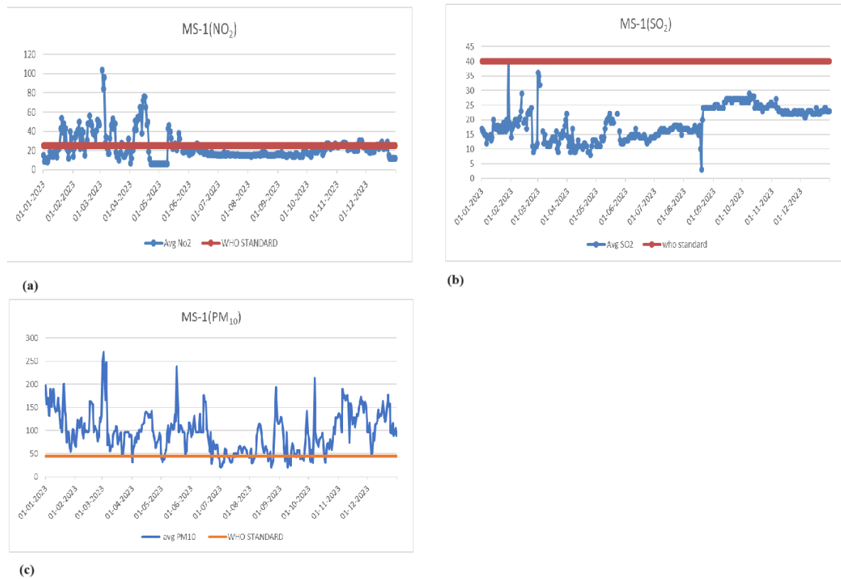
Figure 4. Comparative prediction of ground truth (a) NO_2 ,(b) SO_2 and (c) PM_{10} with WHO standards of MS-1
